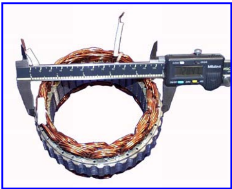
E Total Outside Diameter
