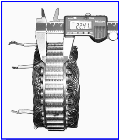
B Exposed Thickness
